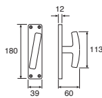
Art. 00252 CREMONESE (meccanismo a precisare) Window handle with mechanism
